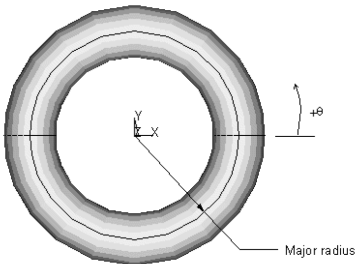
Figure 5.16 Torus Primitive
