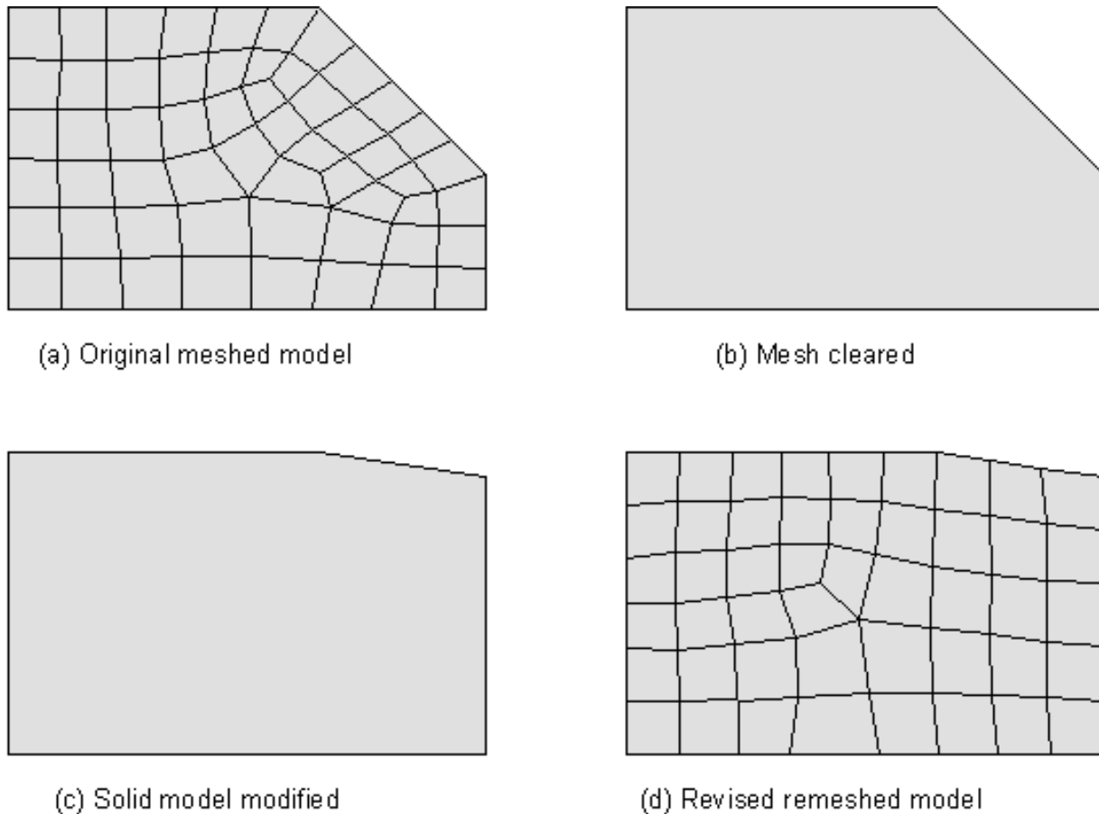
Figure 5.8 Revising a Meshed Solid Model
