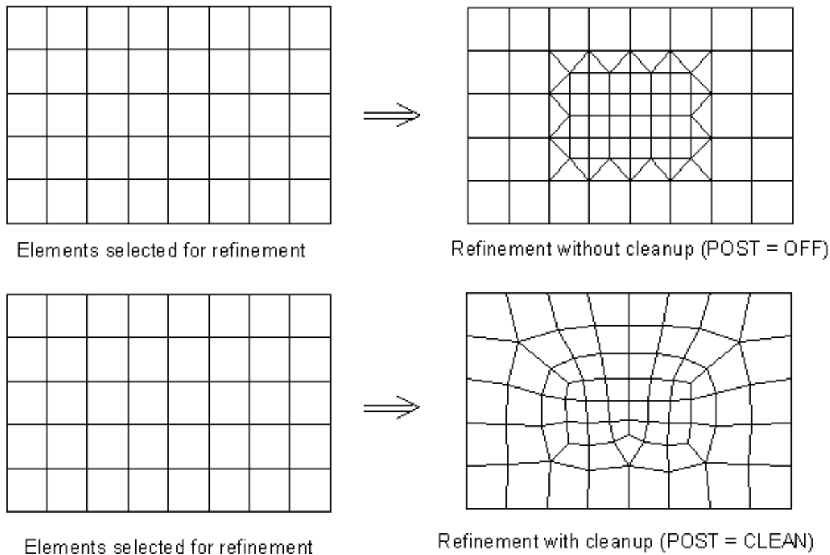
Figure 8.3 All-Quadrilateral Mesh
