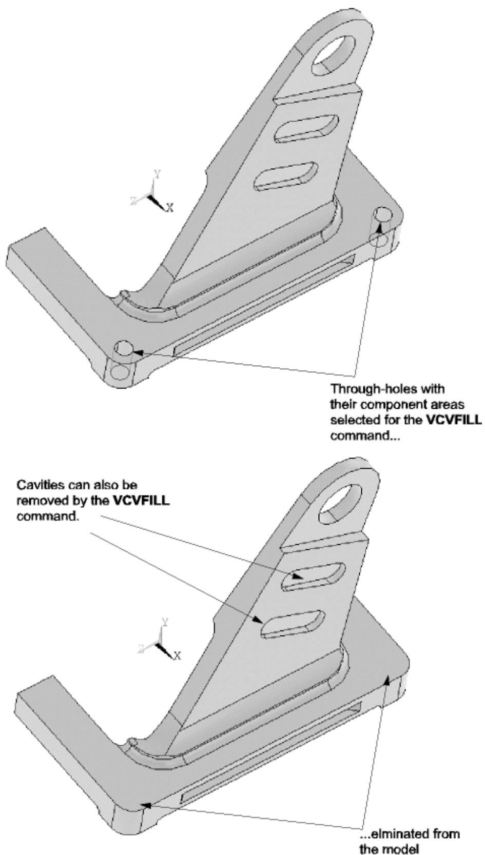
Figure 6.10 Two Through-Holes Removed by the VCVFILL Command
