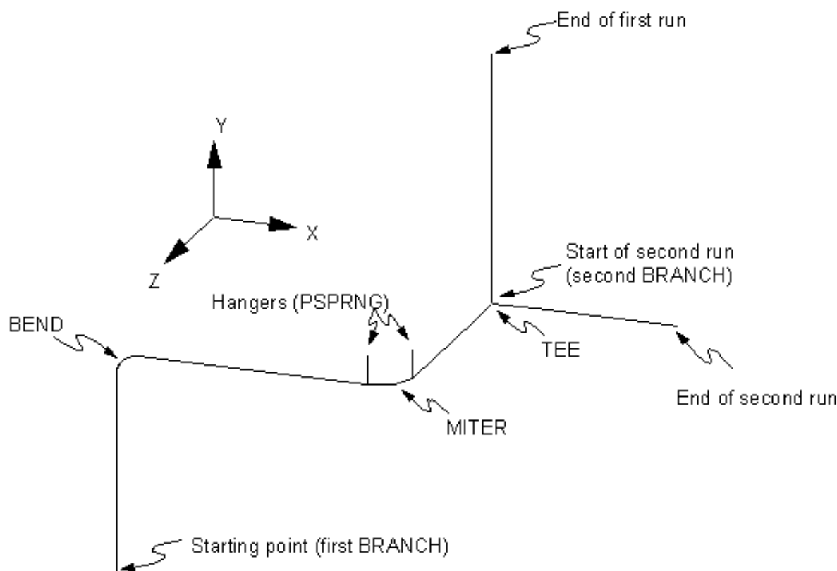
Figure 10.1 Sample Piping Input
