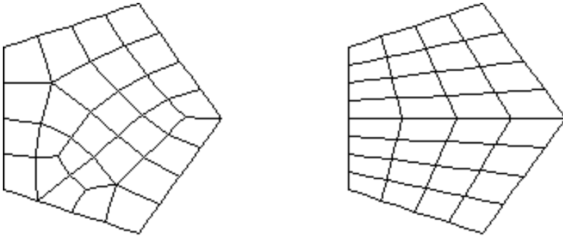
Figure 5.6 Free and Mapped Meshes
