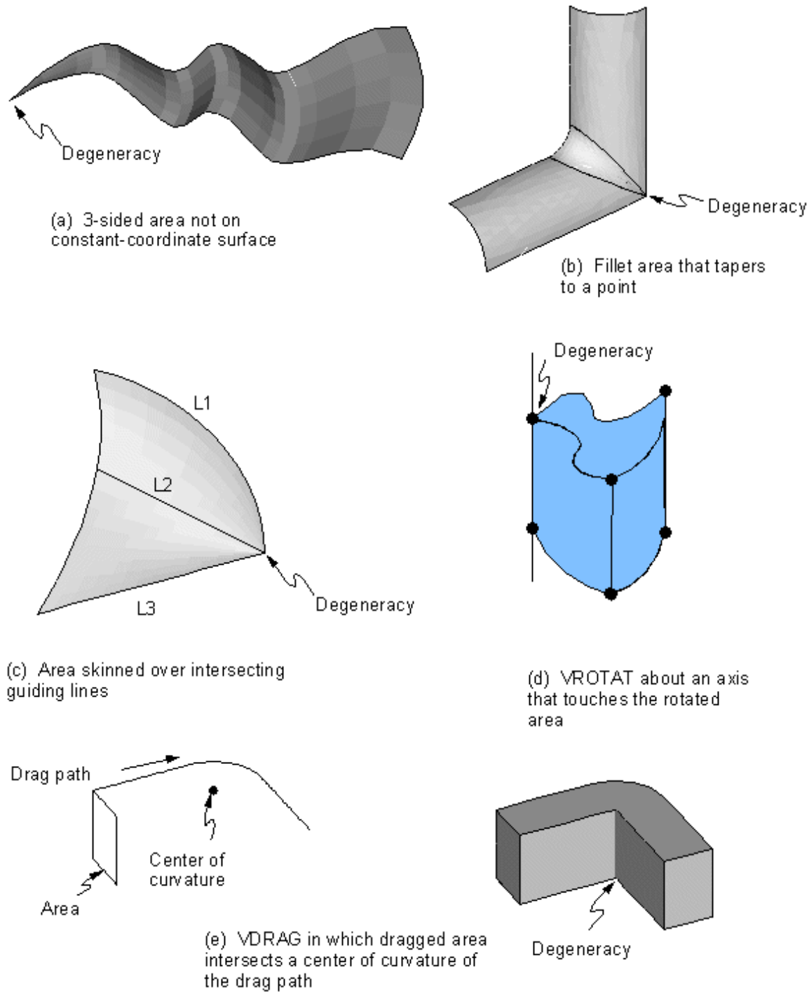
Figure 5.65 Examples of Degeneracies
