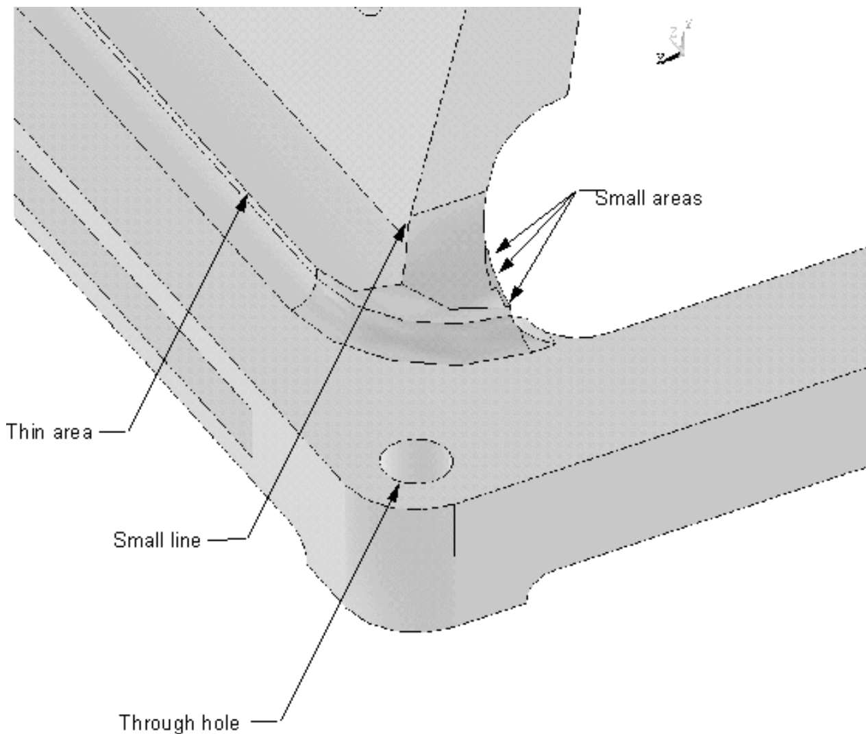
Figure 6.1 Meshing Problems
