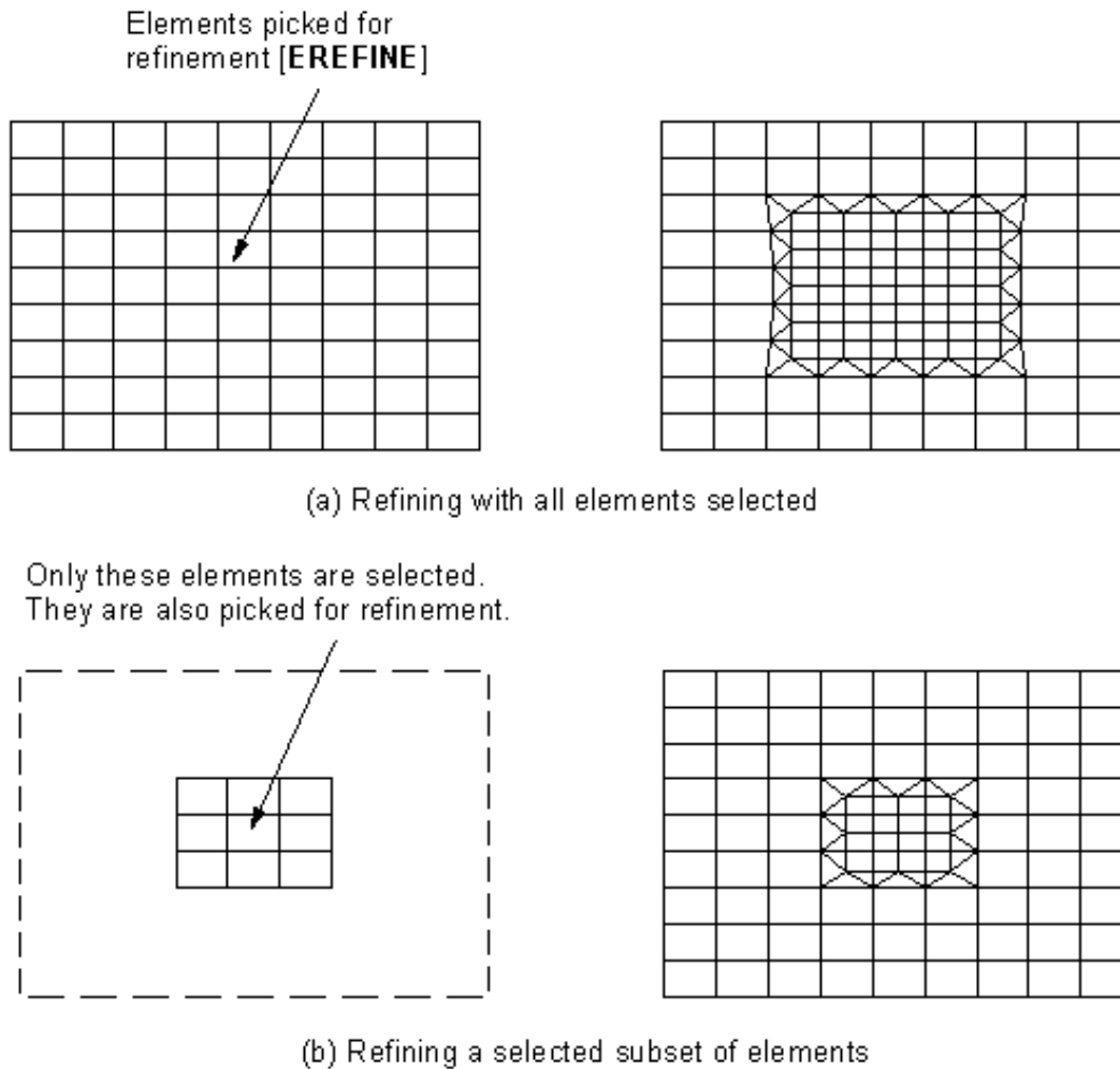
Figure 8.6 Only Selected Elements are Refined
