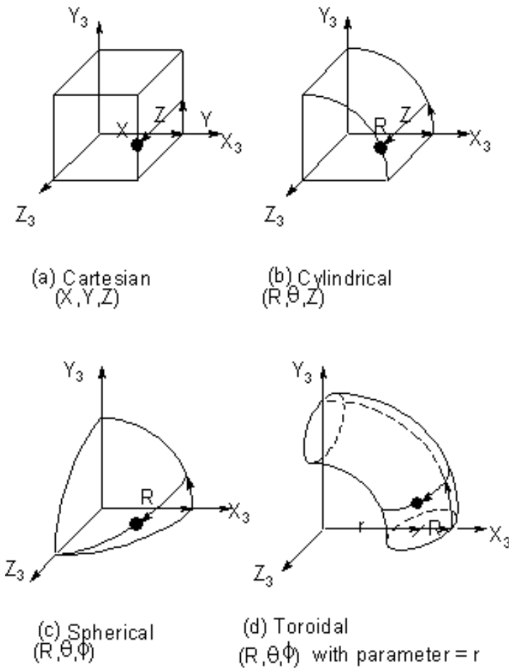
Figure 3.3 Coordinate System Types
