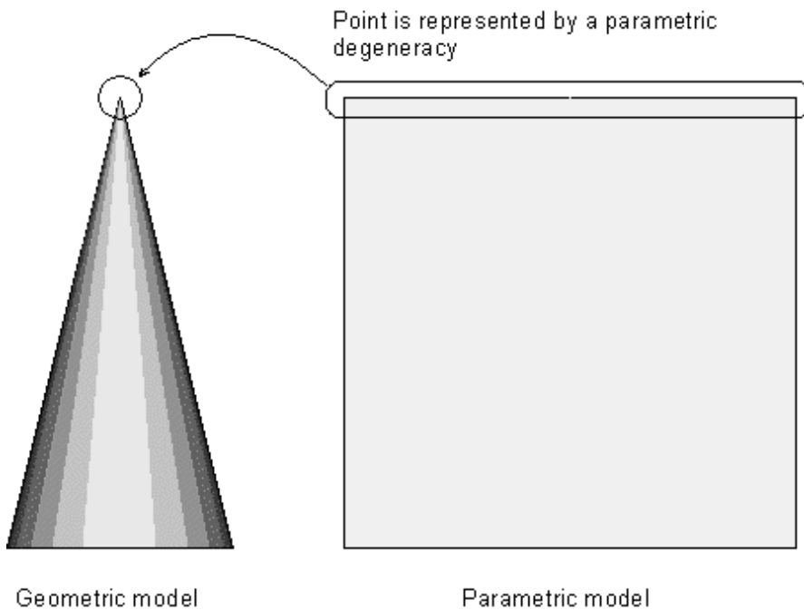
Figure 5.63 Cone Surface Maps to a Parametric Square
