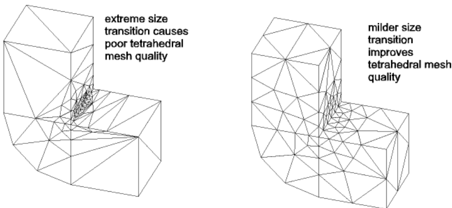
Figure 7.41 Avoiding Extreme Element Size Transitions
