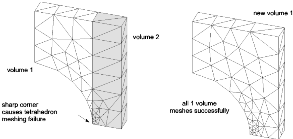
Figure 7.40 Avoiding Sharp Corners
