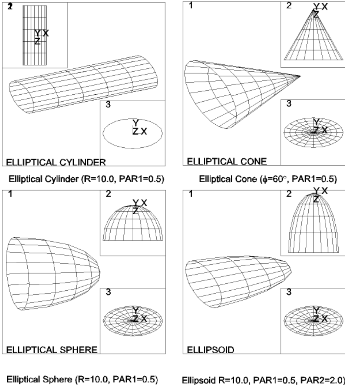
Figure 3.5 Meshed Surfaces of Constant Value
