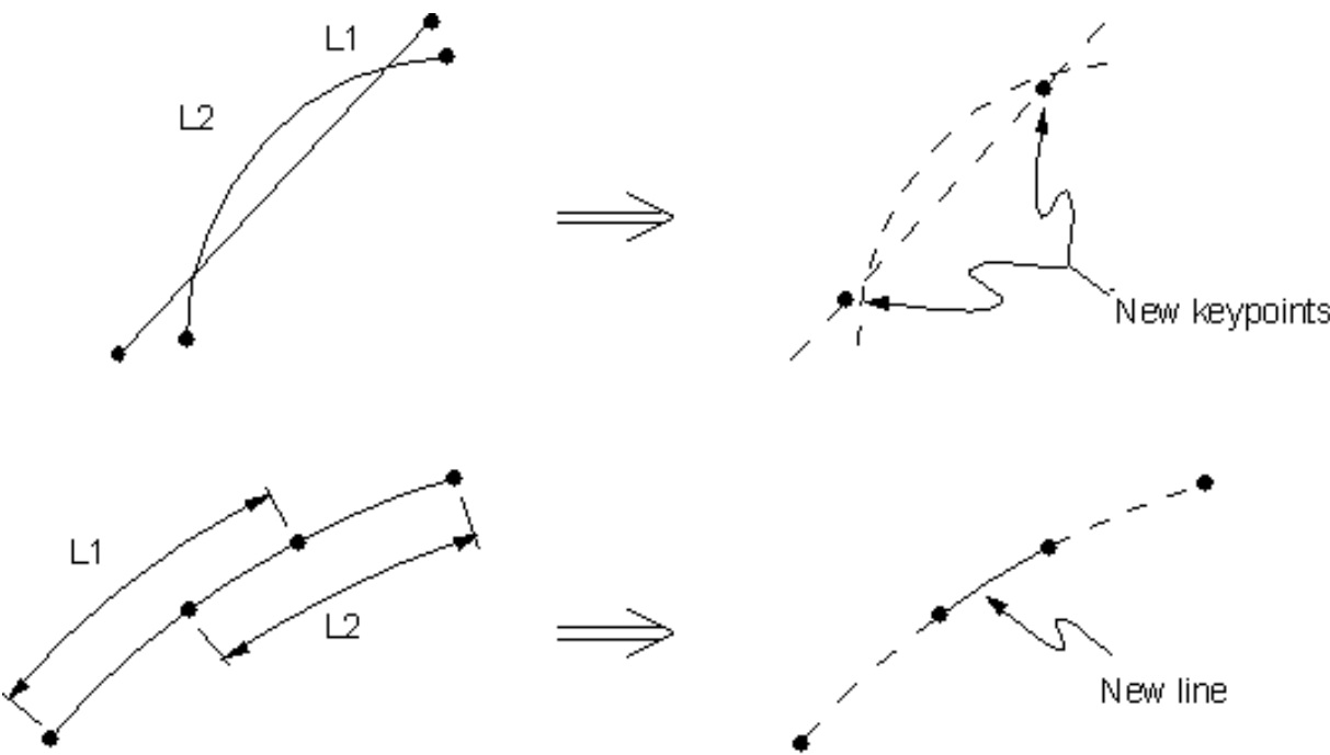
Figure 5.19 LINL (Line Intersect Line)
