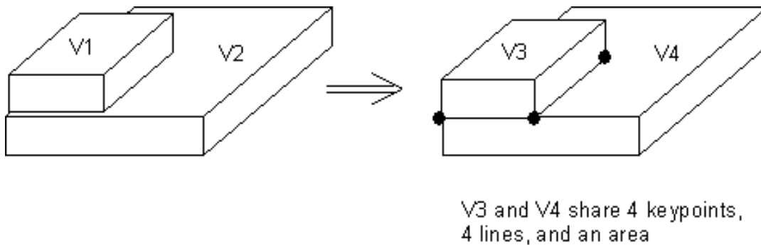
Figure 5.58 VGLUE (Volume Glue Volume)
