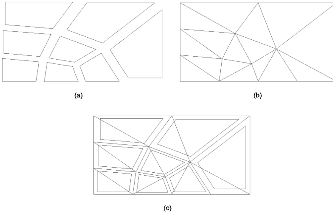
Figure 7.25 Mapped Meshes
